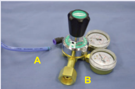
Propellant gas line connection
